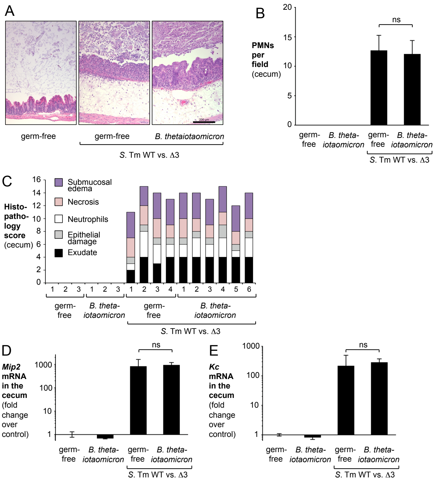
Figure S4: Cecal inflammation induced by S. Tm in a gnotobiotic mouse model. Related to Fig. 6. Germ-free animals and mice mono-associated with B. thetaiotaomicon were mock-treated or infected with S. Tm as shown in Fig. 6 and cecal inflammation analyzed. (A) Representative images of hematoxylin and eosin-stained sections. (B) Infiltration of the cecal mucosa with PMNs. A total number of 10 fields were counted per individual animal. Bars represent the mean \pm standard error. ns, not statistically significant. (C) Semi-quantitative histopathology score for the cecum. Each bar represents one animal. (D and E) mRNA levels of the CXC chemokines MIP-2 (D) and KC (E) in the cecal tissue as determined by RT-qPCR. Bars represent the geometric mean \pm standard error. ns, not statistically significant.
